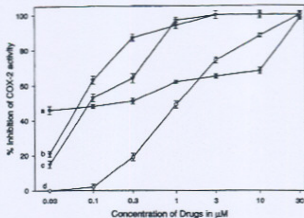
FIG. 2. The inhibitory effect of (a) phycocyanin, (b) rofecoxib, (c) celecoxib, and (d) indomethacin (0.03–30.0 \mu M) on human recombinant COX-2 activity. The results are expressed as % inhibition of COX-2 activity by inhibitors. The experimental details are as described under Materials and Methods.
