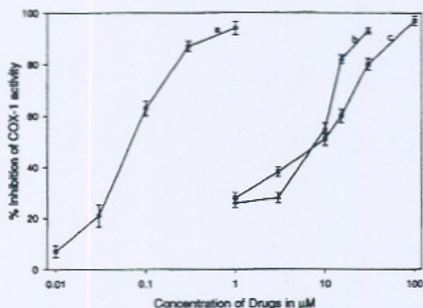
FIG. 1. The inhibitory effect of (a) indomethacin (0.01–1.0 \mu M), (b) phycocyanin (1.0–30.0 \mu M), and (c) celecoxib (1.0–100 \mu M) on ram seminal vesicle COX-1 activity. The results are expressed as % inhibition of COX-1 activity by inhibitors. The experimental details are as described under Materials and Methods.
